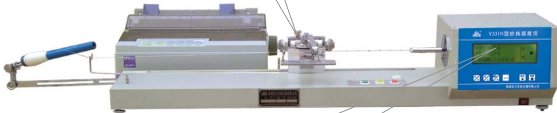
GRIP WITH PRE-TENSION DEVICE
